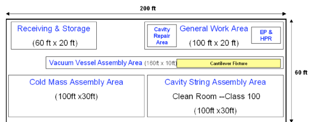
Figure 6 SMTF cryomodule assembly facility plan.
