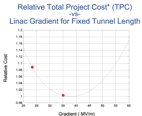
Fig. 1 Estimated Cost vs. gradient [5]
