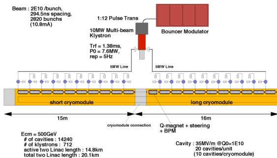
Figure 4 RF unit configuration of ILC main linac.
