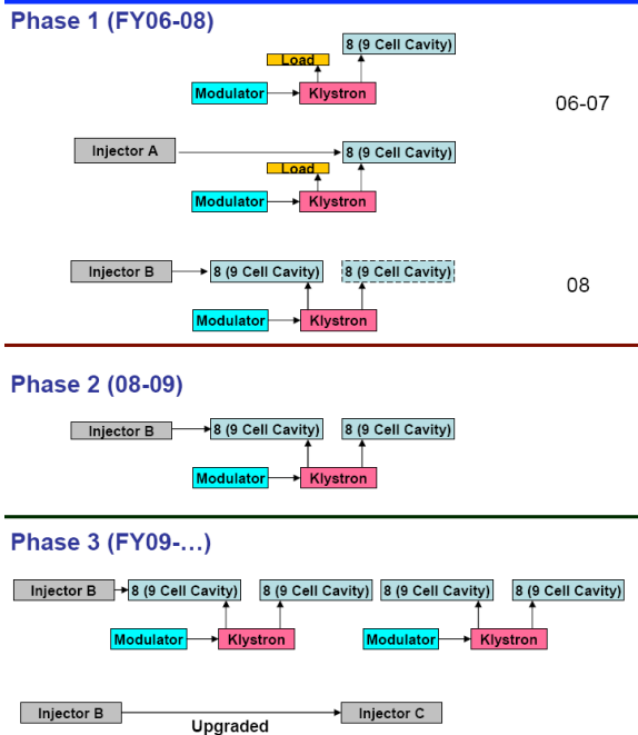
Figure 5 SMTF 3 steps for ILC module test.
