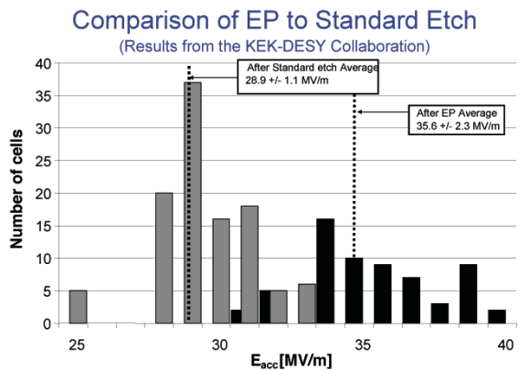
Figure 2 Accelerating gradient by EP process [6]
